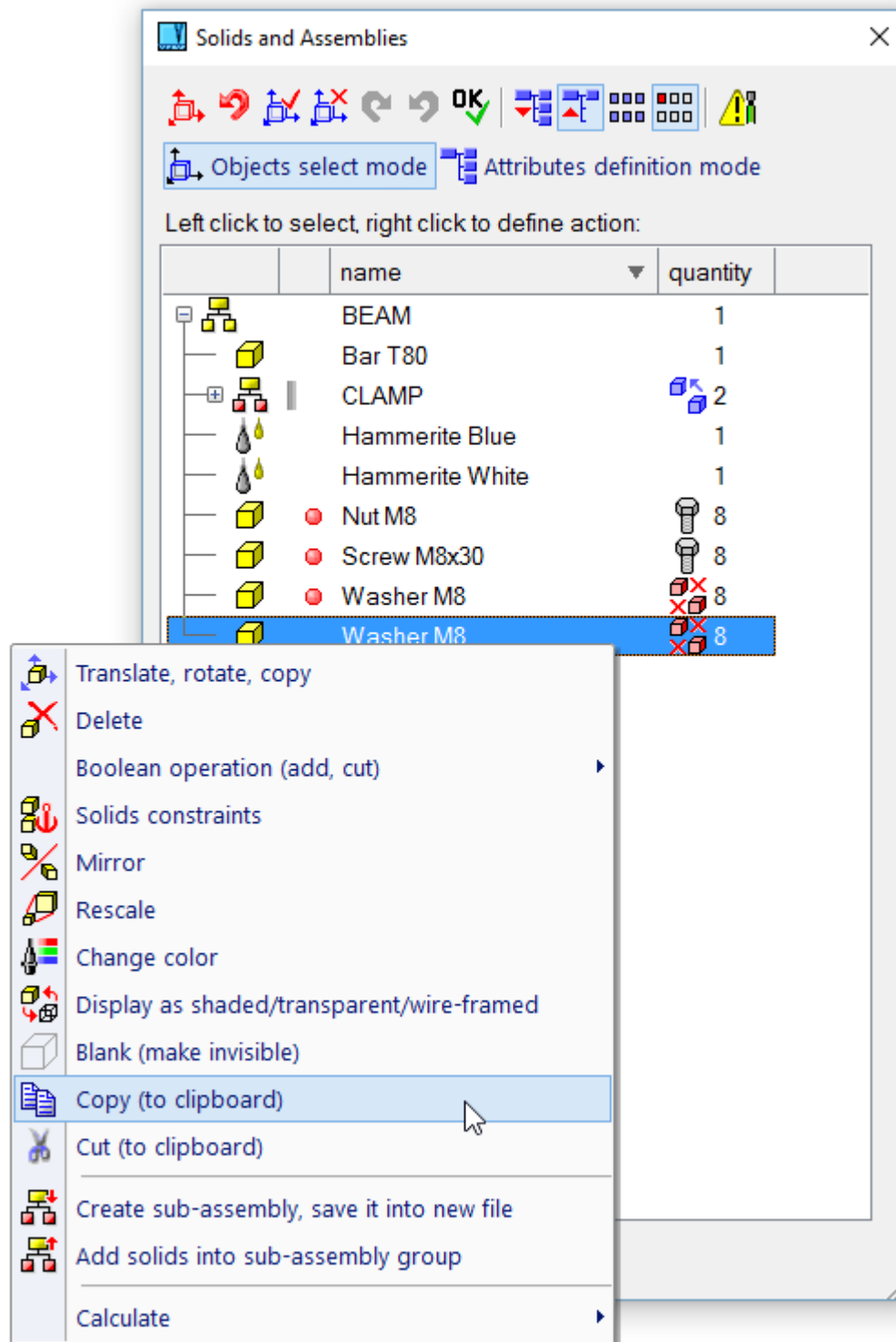
Assembly tree structure, objects select mode
