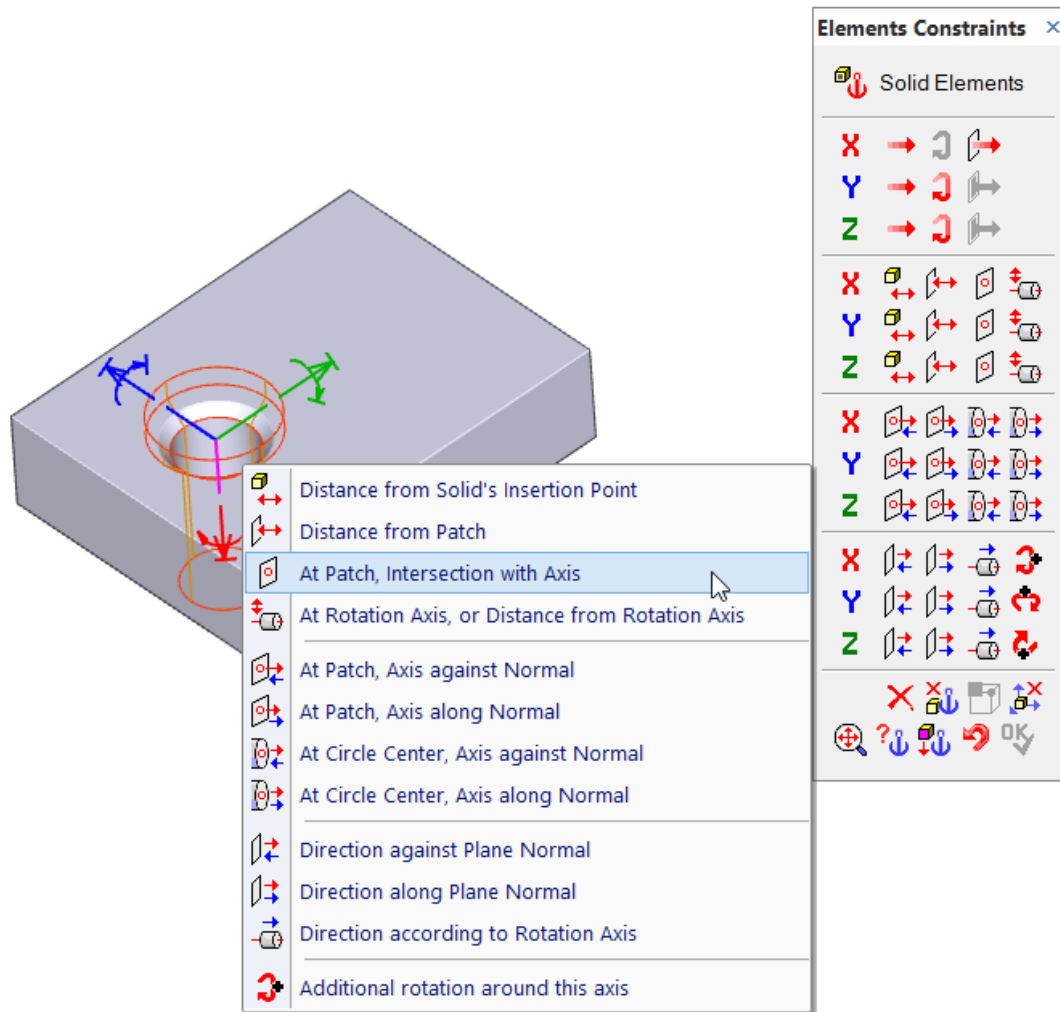
Constraint definition, Constraint panel
