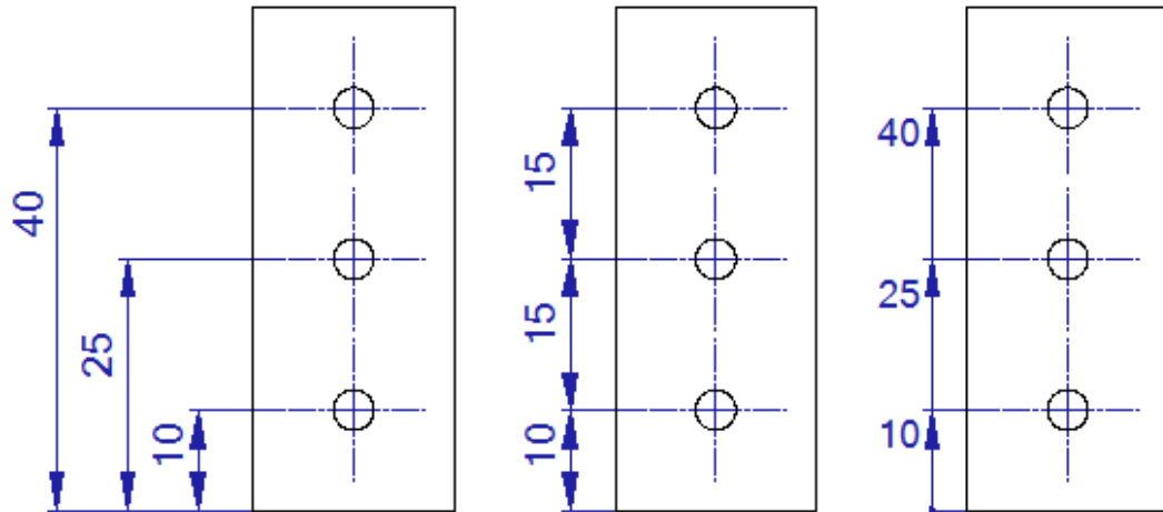
Example of baseline, serial and datum dimensions
