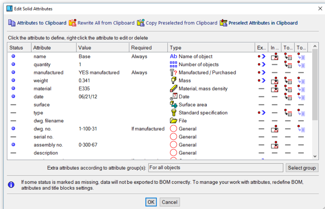
Solid attributes definition
