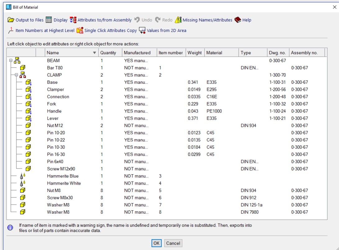
Bill of materials, created as complete assembly structure
