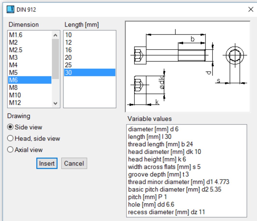
Mechanical part selection - 2D screw (bolt)
