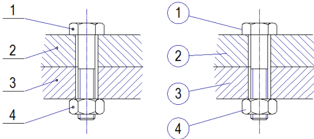
Example of leaders
